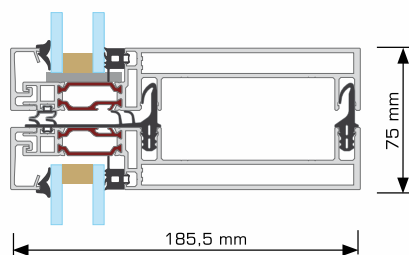
Transom cross-section
