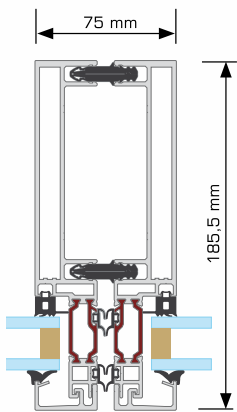
Mullion cross-section
